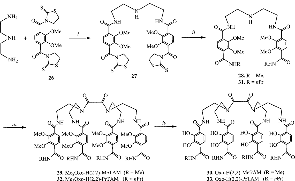
Scheme 3. Synthesis of octadentate oxo-catecholamide ligands; reagents and conditions 2: (i) CH 2 Cl 2 containing 2% MeOH; (ii) NH 2 Me, MeOH, room temp., 4 h; (iii) Et 3 N, anhydrous THF, oxalyl chloride, -30 °C; (iv) 1. BBr 3 , CH 2 Cl 2 , -78 °C, under Ar; 2. MeOH, -78 °C; 3. H 2 O, 100 °C
