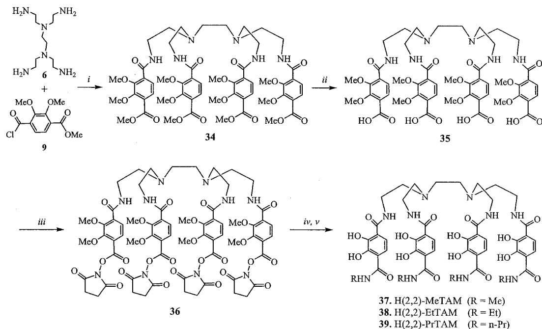
Scheme 4. Synthesis of octadentate 2,3-dihydroxyterephthalamide ligands; reagents and conditions: (i) 1. anhydrous THF, Et 3 N, under N 2 ; 2. under N 2 , room temp., 12 h; (ii) 1. aqueous workup, MeOH, 1 M NaOH; 2. 100 °C, 4 h; 3. H 2 O, 6 M HCl; (iii) THF, -10 °C, under Ar, N -hydroxysuccinimide, 1,3-dicyclohexylcarbodiimide; (iv) 24 h, room temp., THF, RNH 2 ; (v) 1. BBr 3 , CH 2 Cl 2 , -78 °C, under Ar; 2. MeOH, -78 °C; 3. H 2 O, 100 °C
