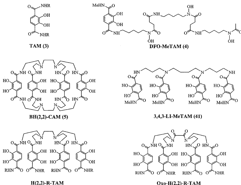
Figure 2. Octadentate terephthalamide ligands
