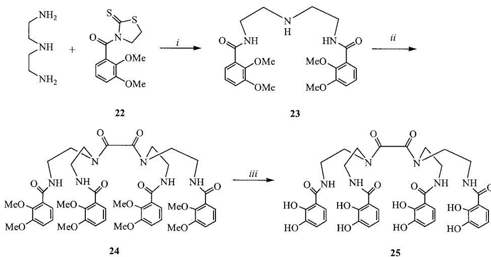
Scheme 2. Synthesis of octadentate oxo-catecholamide ligands 1 , Oxo-H(2,2)-CAM; reagents and conditions: (i) anhydrous THF, \text{Et}_3\text{N} ; (ii) 1. \text{Et}_3\text{N} , anhydrous THF, oxalyl chloride, -78^\circ\text{C} ; 2. 25^\circ\text{C} , 4 h; 3. \text{CH}_2\text{Cl}_2 , aqueous workup, 1 M HCl; (iii) 1. \text{BBr}_3 , \text{CH}_2\text{Cl}_2 , -78^\circ\text{C} , under Ar; 2. MeOH, -78^\circ\text{C} ; 3. \text{H}_2\text{O} , 100^\circ\text{C}
