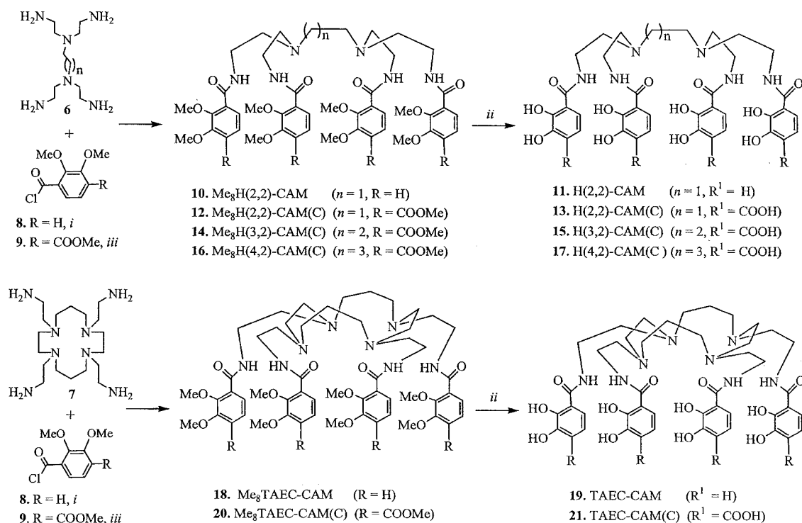
Scheme 1. Synthesis of octadentate catecholamide ligands; reagents and conditions: (i) \text{CH}_2\text{Cl}_2 , room temp., 24 h; (ii) 1. \text{BBr}_3 , \text{CH}_2\text{Cl}_2 , -78^\circ\text{C} , under Ar; 2. MeOH, -78^\circ\text{C} ; 3. \text{H}_2\text{O} , 100^\circ\text{C} (iii) anhydrous THF, \text{Et}_3\text{N}
