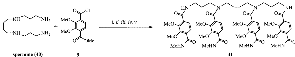
Scheme 5. Synthesis of 3,4,3-LiMeTAM; reagents and conditions: (i) 1. anhydrous THF, under N 2 ; 2. under N 2 , room temp., 12 h; (ii) 1. aqueous workup, MeOH, 1 M NaOH; 2. 100 °C, 4 h; 3. H 2 O, 6 M HCl; (iii) THF, -10 °C, under Ar, N -hydroxysuccinimide, 1,3-dicyclohexylcarbodiimide; (iv) 24 h, room temp., THF, MeNH 2 ; (v) 1. BBr 3 , CH 2 Cl 2 , -78 °C, under Ar; 2. MeOH, -78 °C; 3. H 2 O, 100 °C
