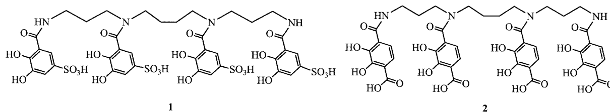
Figure 1. Tetracatecholate ligands 3,4,3-LICAM(S) (1) and 3,4,3-LICAM(C) (2)
